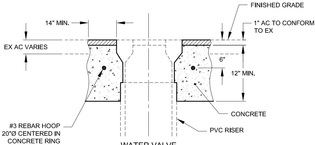
WATER VALVE (MONUMENT BOX SIMILAR)
